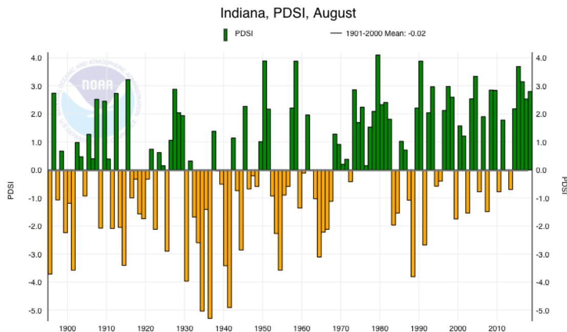
Figure 14. Values for the Palmer Drought Severity Index for Indiana, 1895 – 2017
