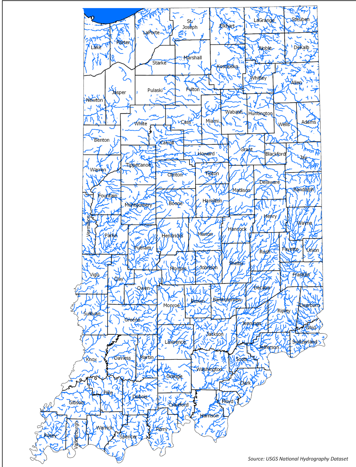
Figure 6. Perennial Streams
