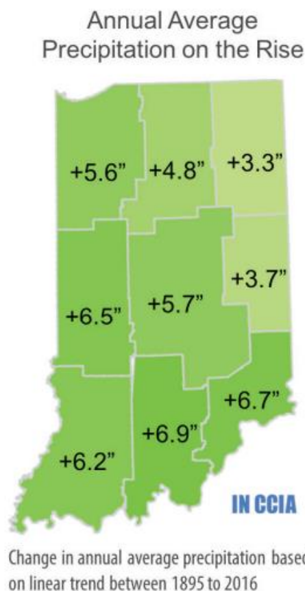
Figure 20. Average Precipitation Increase (Widhalm M. H., 2018)
