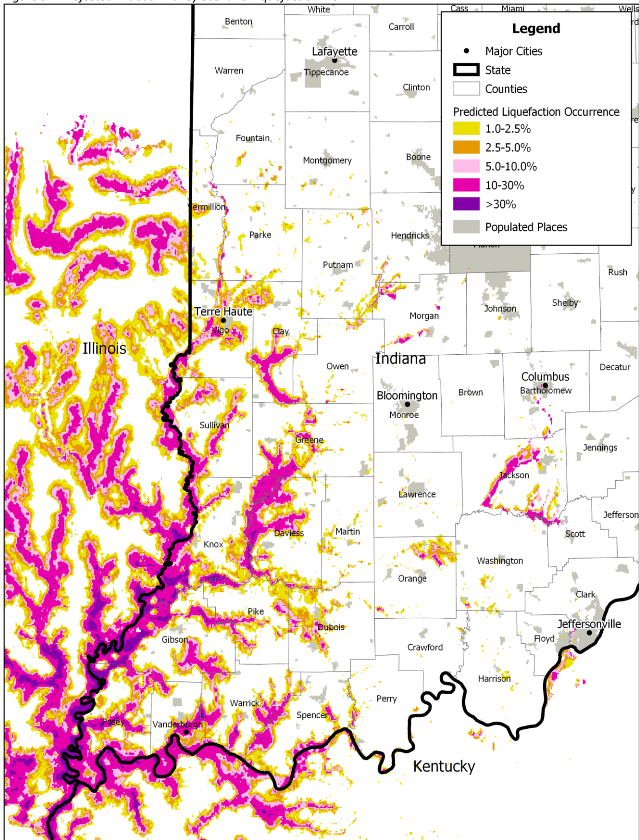
Figure 91. Projected Wabash Valley Scenario Liquefaction Risk
