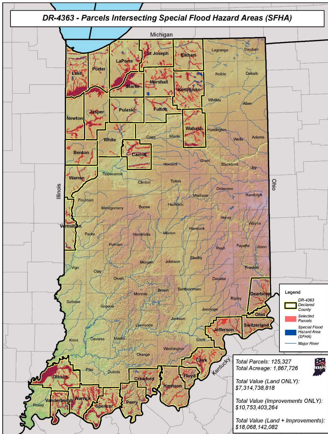
Figure 41. 2018 Flood Extent
