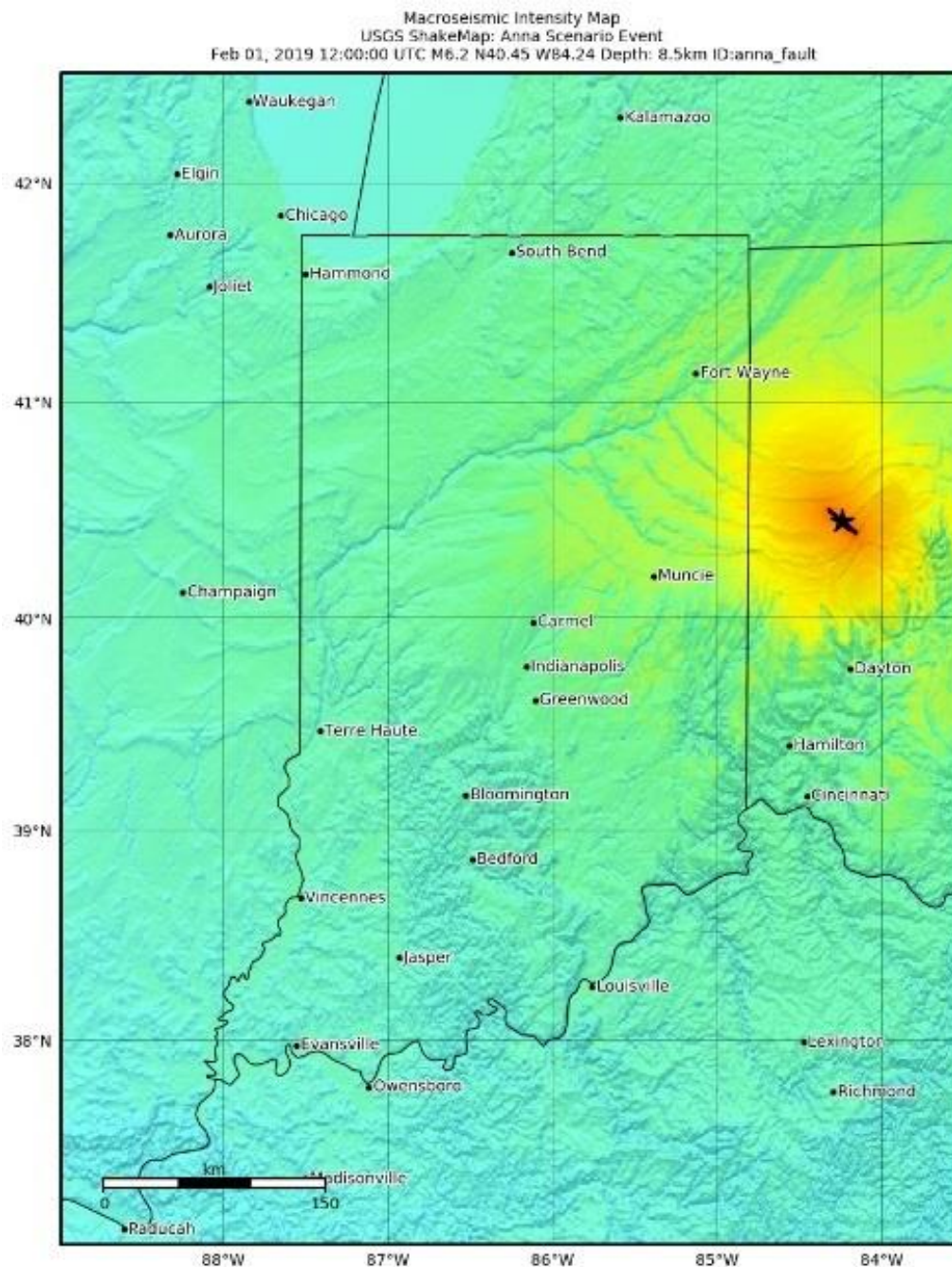
Figure 92. Projected Anna, Ohio Scenario Intensity map
