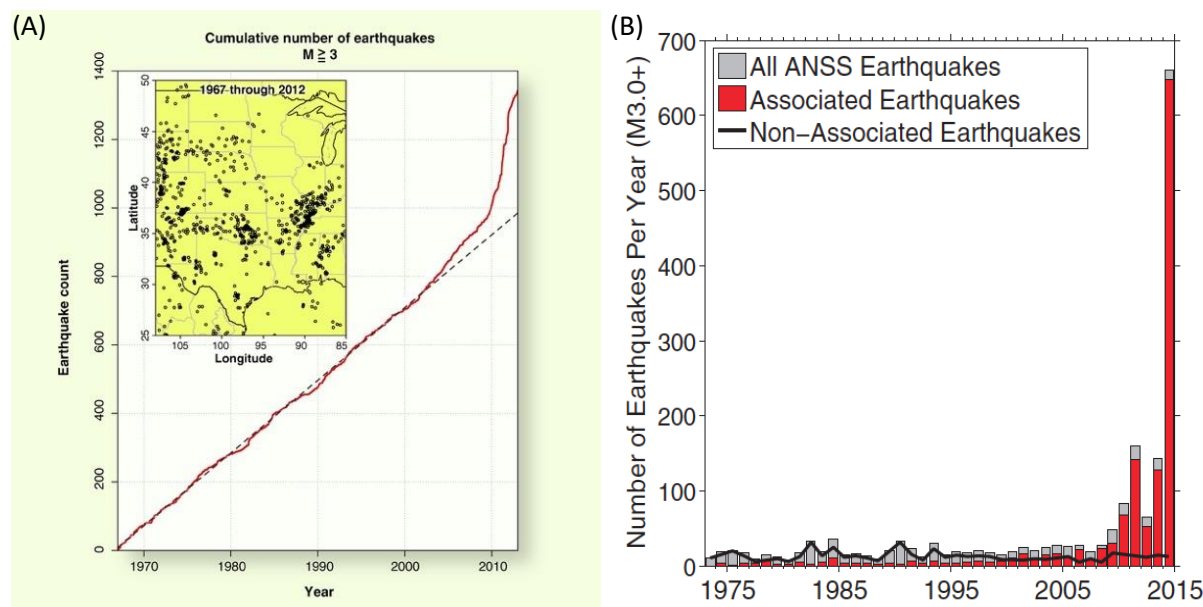
Figure 129. Induced Earthquakes in the Central United States
