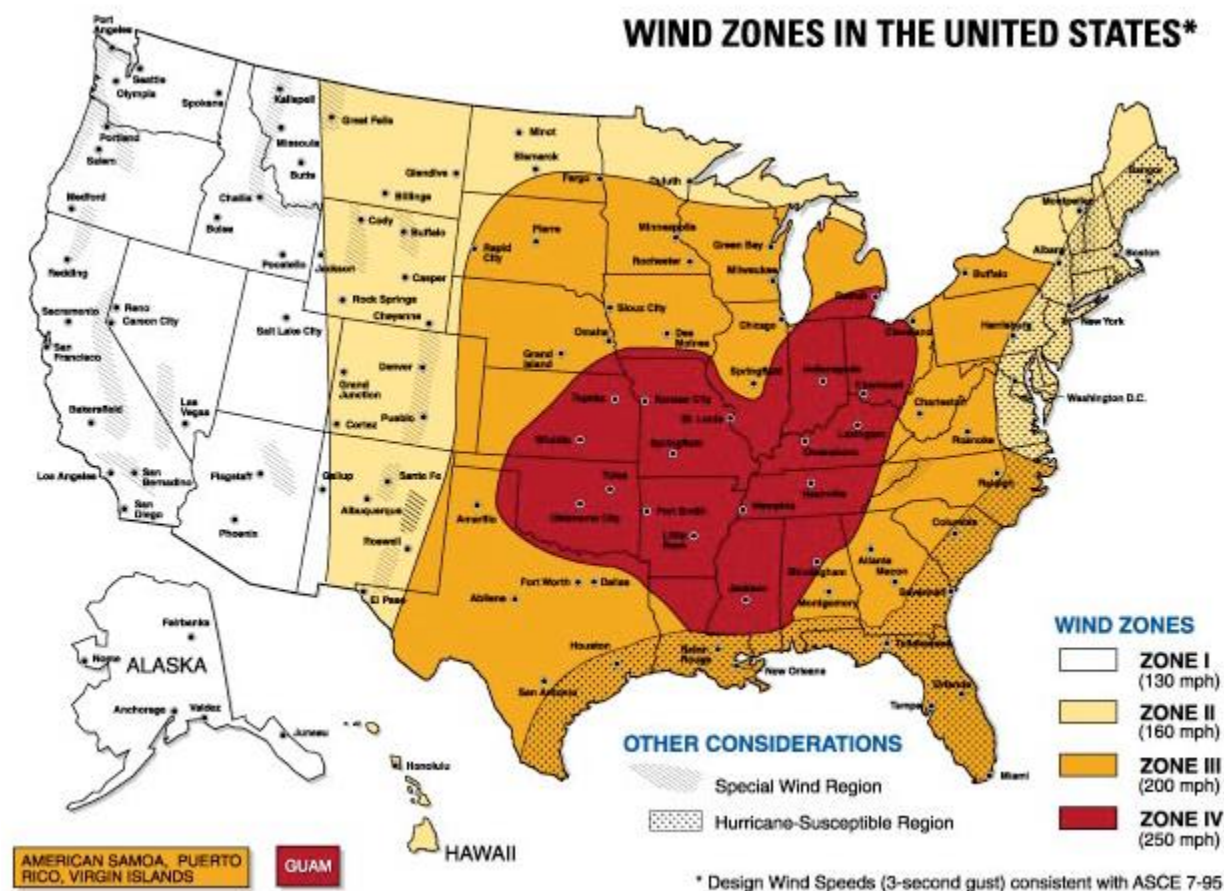
Figure 62. Wind Zones in the United States (FEMA)
